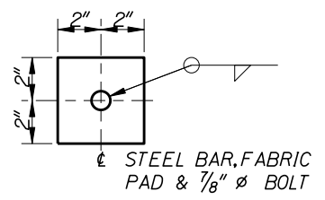
SECTION C 3"=1'-0"
