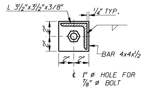
SECTION B 3"=1'-0"
