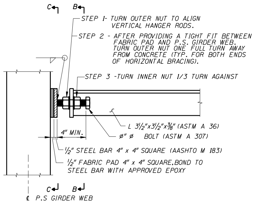
DETAIL A 3"=1'-0"
