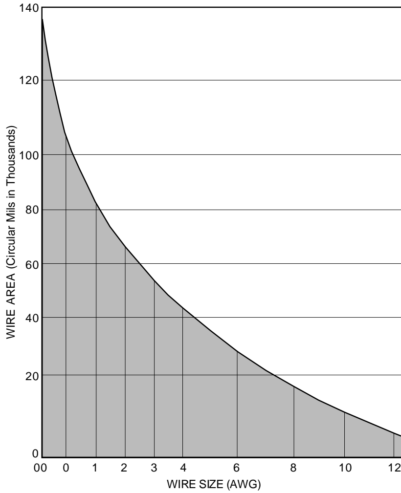
Figure 355.02.02-02 Wire Area vs. Wire Size
