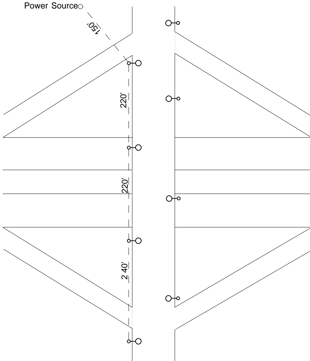
Figure 355.02.02-01 Multiple Lighting System Continuous Conduit
