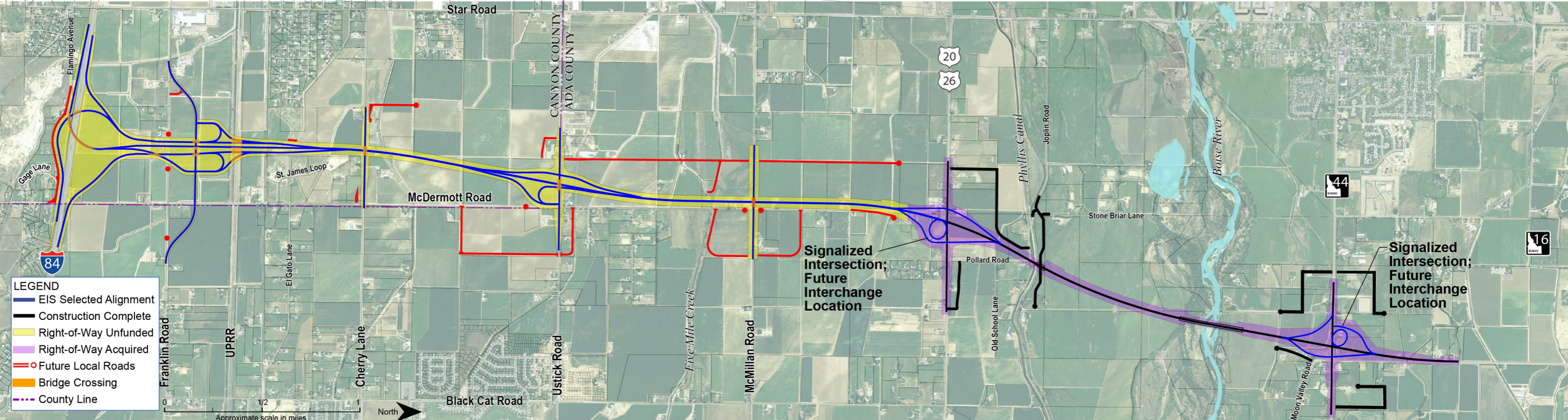
Idaho 16 Selected Alternative Plan View
